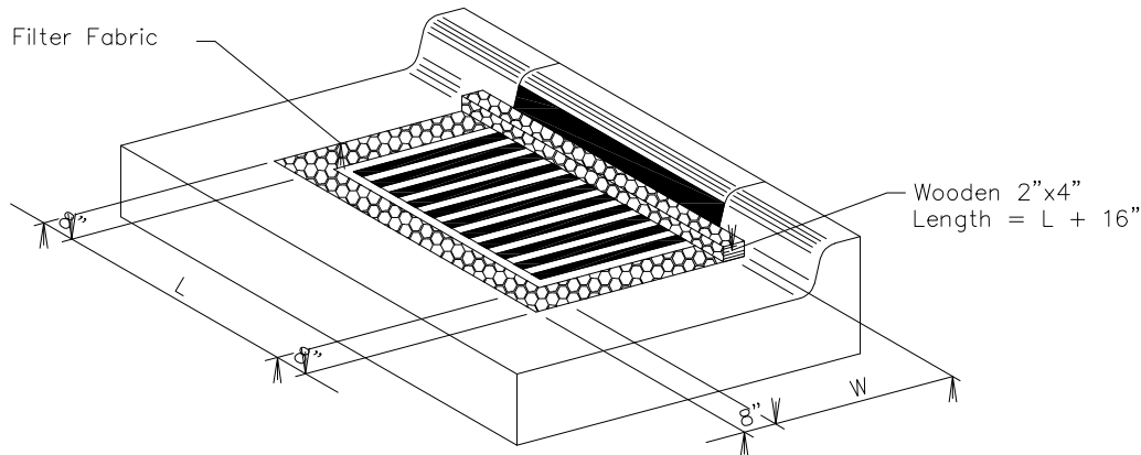
ISOMETRIC VIEW
