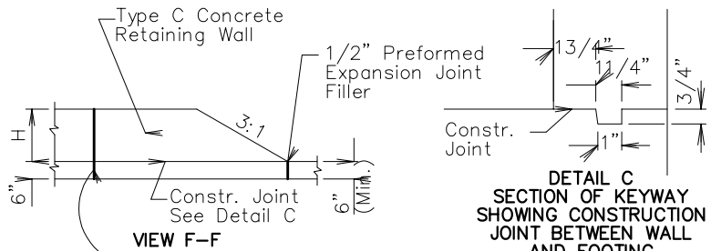
VIEW F-F
