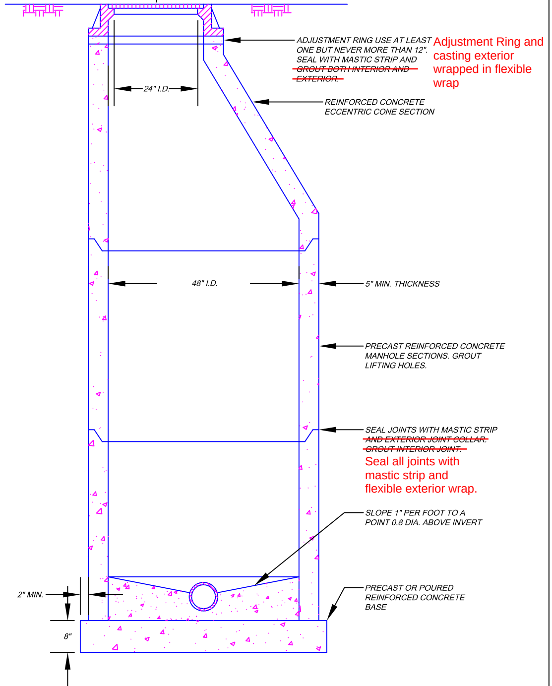
STANDARD SEWER MANHOLE NOT TO SCALE
