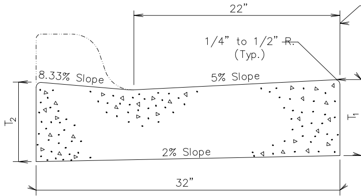
TRANSVERSE SECTION
