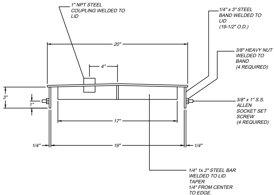
SECTION
