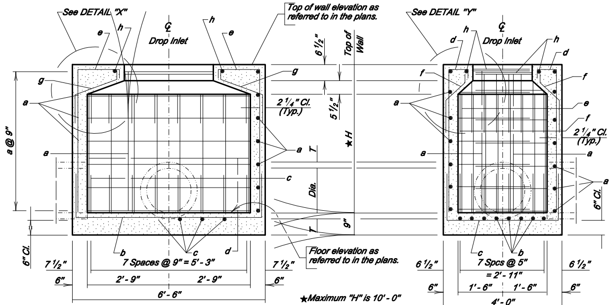
SEC. A - A
