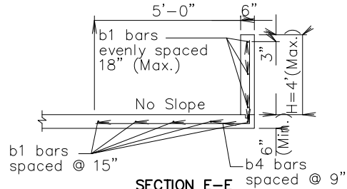
SECTION E-E
