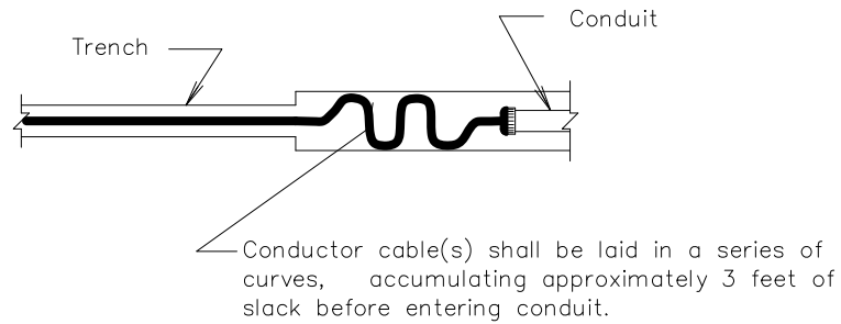
PLAN VIEW
