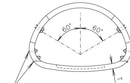
END VIEW
