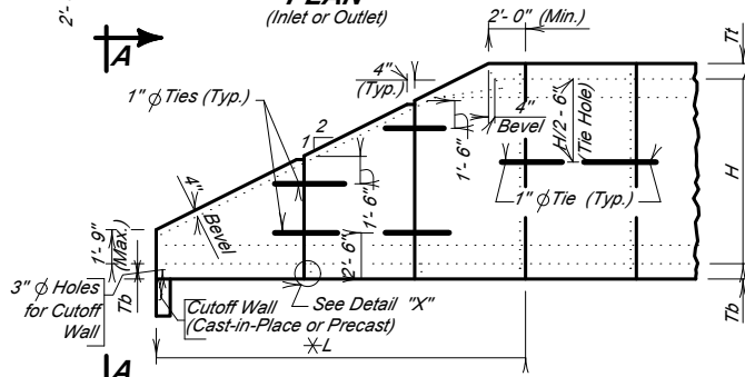
ELEVATION (Inlet or Outlet)
