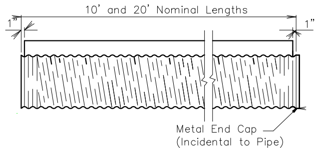
TYPICAL SECTION
