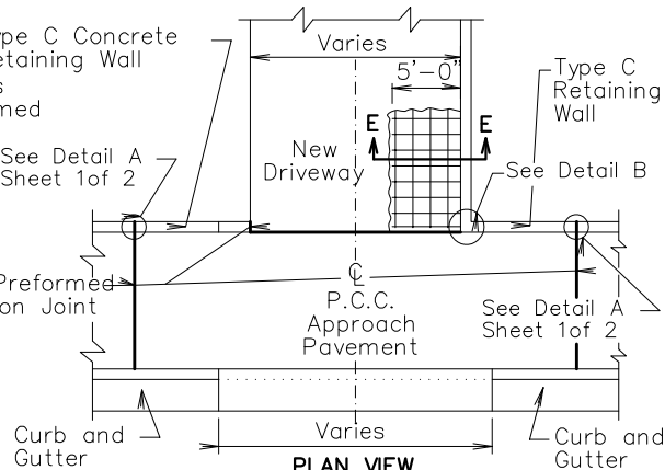
PLAN VIEW TYPE C CONCRETE RETAINING WALL ON P.C.C. DRIVEWAY AND APPROACH PAVEMENT
