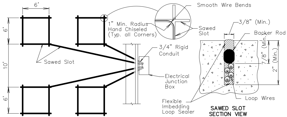
SAWED SLOT LAYOUT
