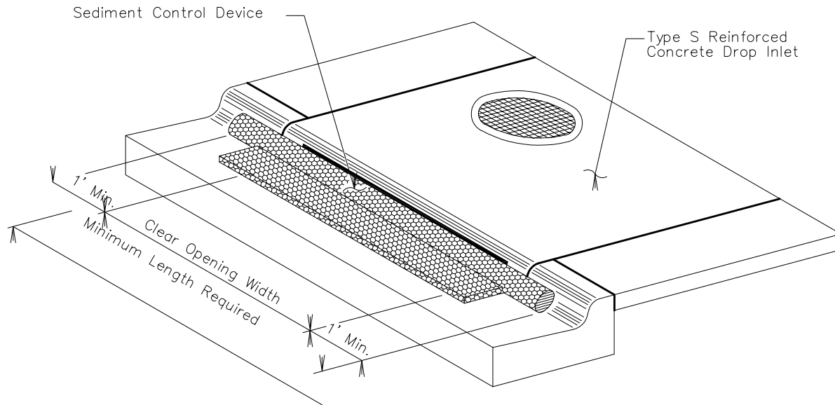
ISOMETRIC VIEW
