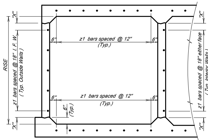
TYPICAL MULTIPLE BARREL VIEW A - A
