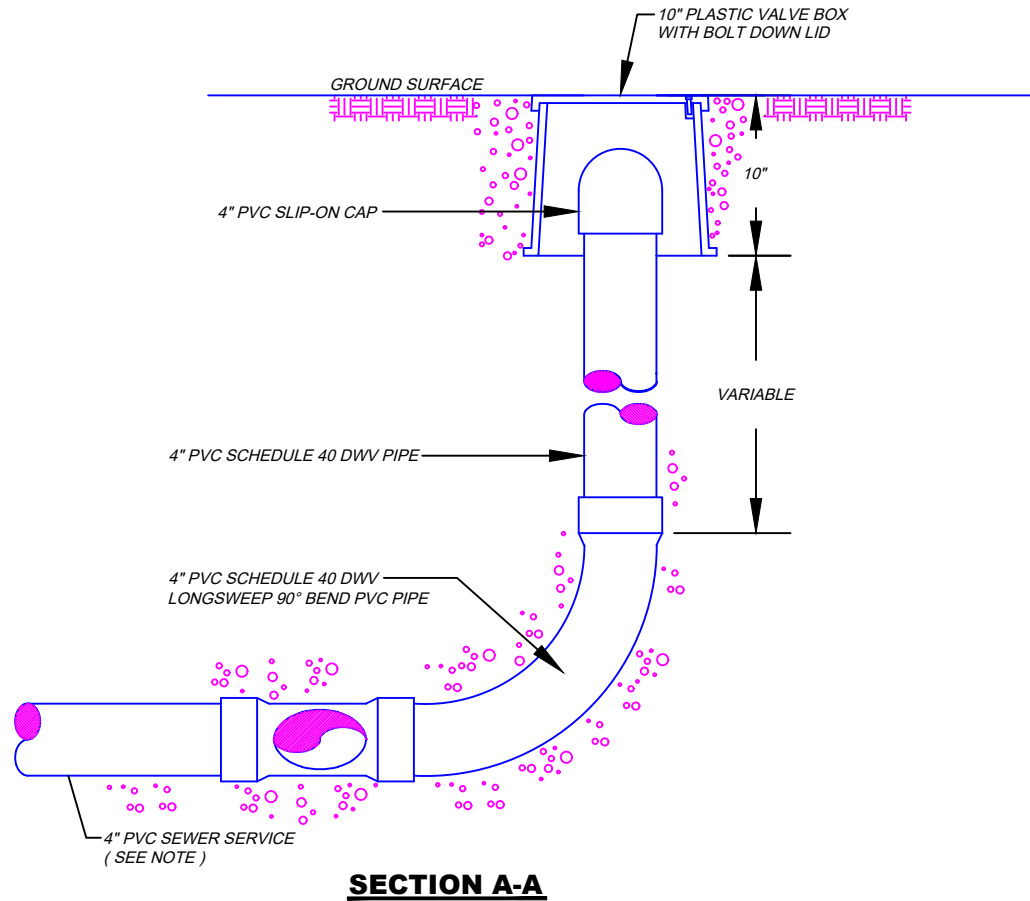
SEWER SERVICE CLEANOUT AT BEND NOT TO SCALE
