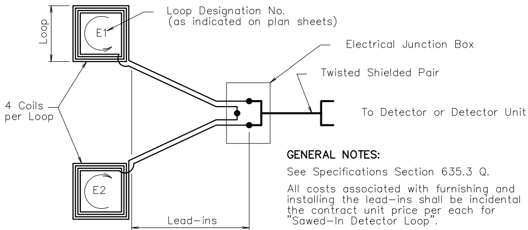
WIRING DIAGRAM
