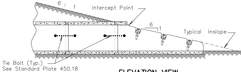
ELEVATION VIEW
