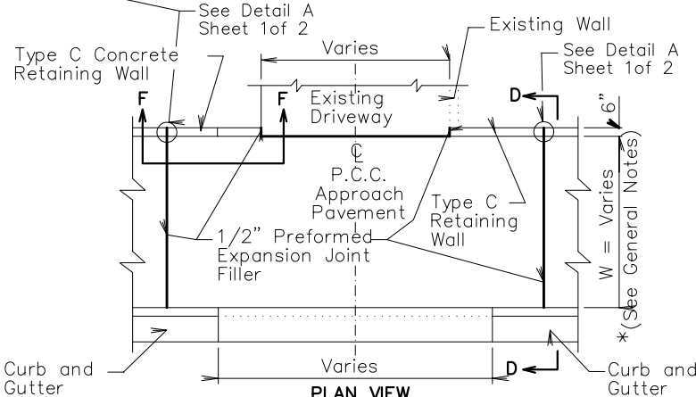
PLAN VIEW TYPE C CONCRETE RETAINING WALL ON P.C.C. APPROACH PAVEMENT
