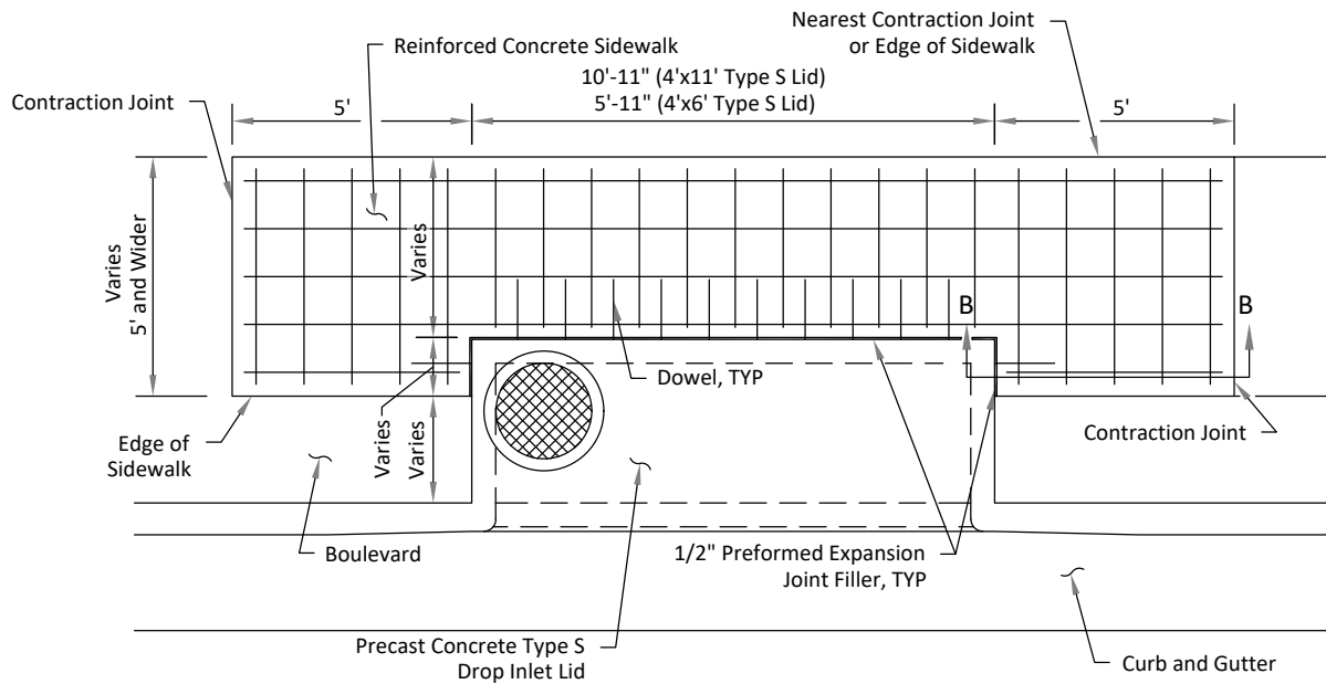
PLAN VIEW (Reinforced Concrete Sidewalk With Boulevard)
