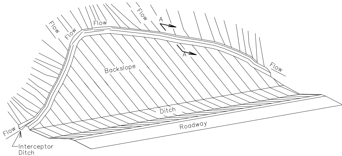
ISOMETRIC VIEW
