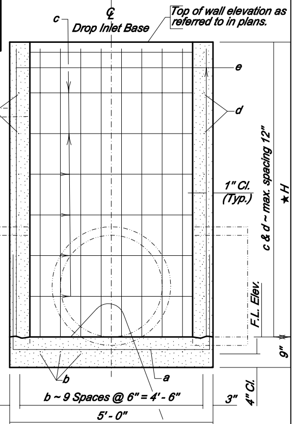
SEC. B - B
